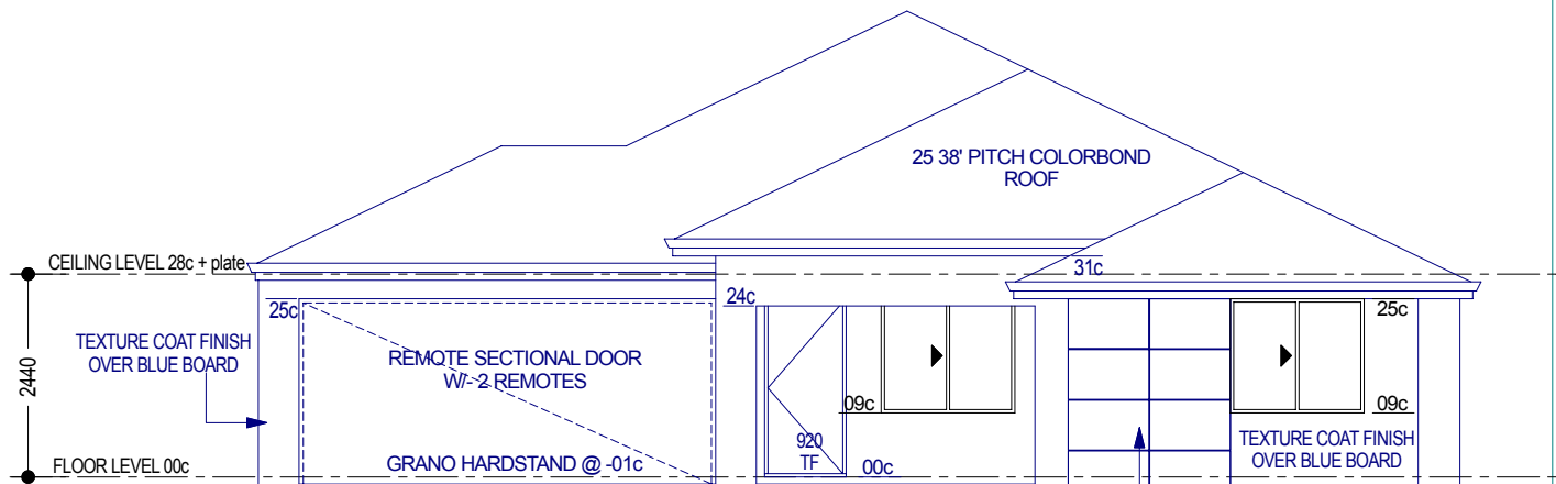
Front Elevation 1:100
