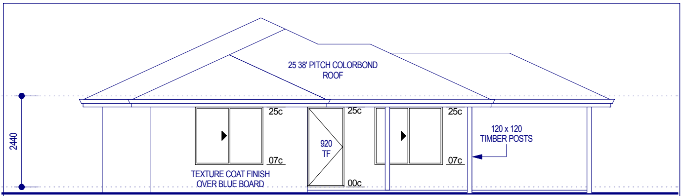
Front Elevation 1:100
