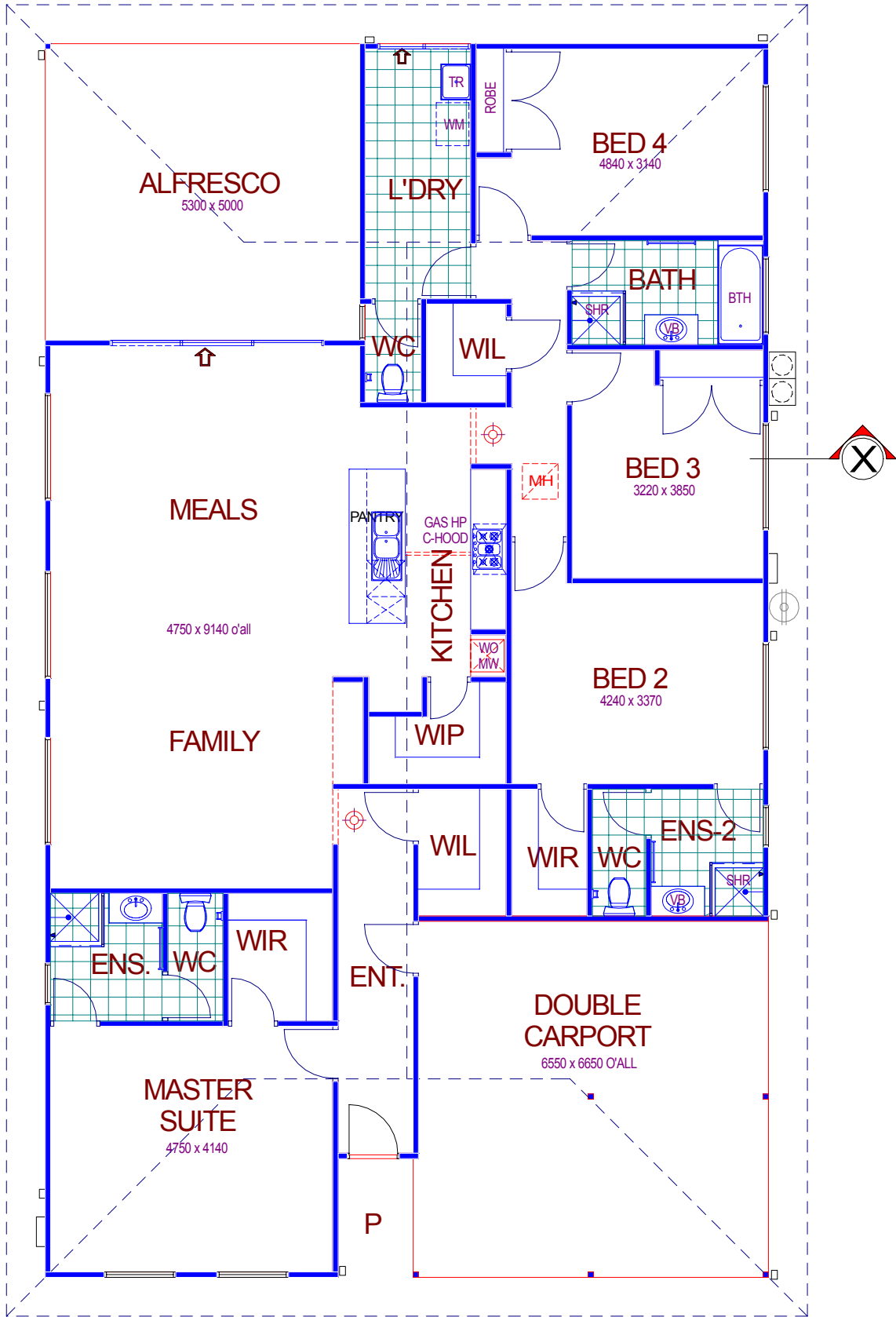
Floorplan 1:100
