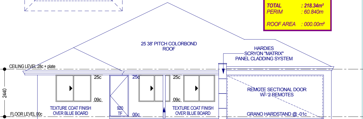
Front Elevation 1:100
